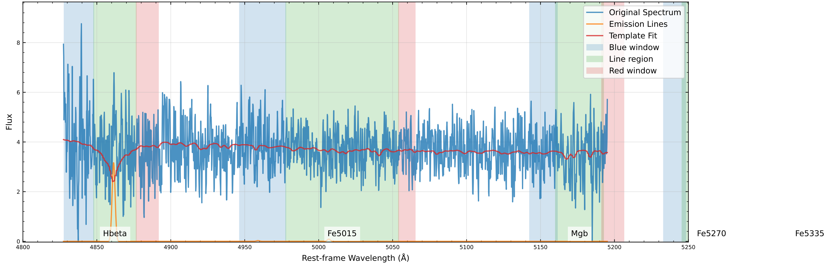
Original Data Comparison (v_star=49.4 km/s, v_gas=27.0 km/s)
