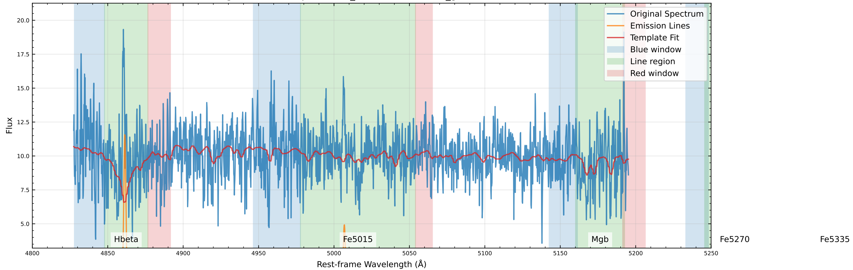
Original Data Comparison (v_star=-59.9 km/s, v_gas=-43.8 km/s)
