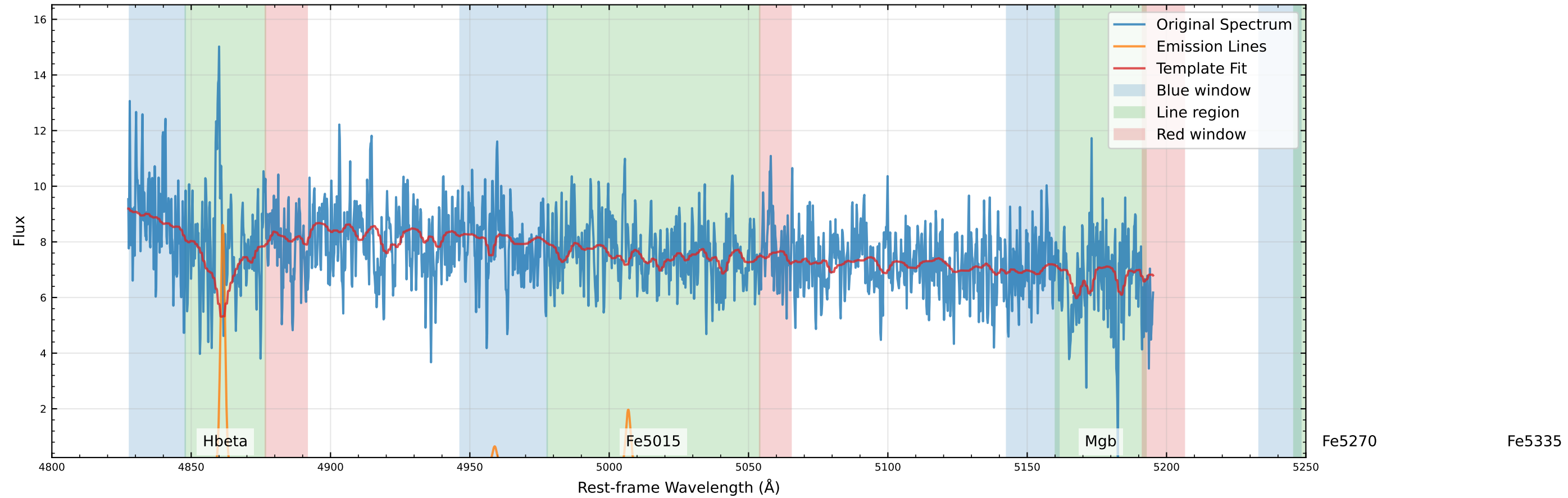
Original Data Comparison (v_star=-101.4 km/s, v_gas=-97.9 km/s)
