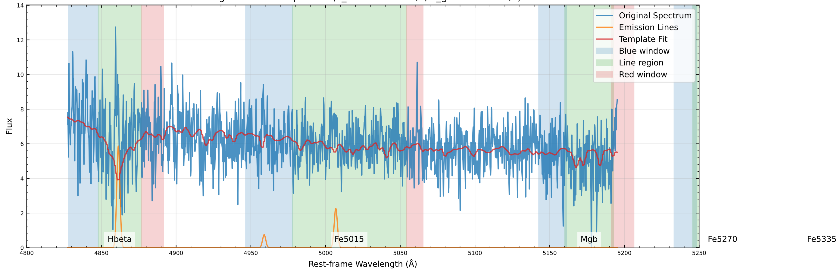
Original Data Comparison ( v_{\text{star}}=-71.6 km/s, v_{\text{gas}}=-73.4 km/s)
