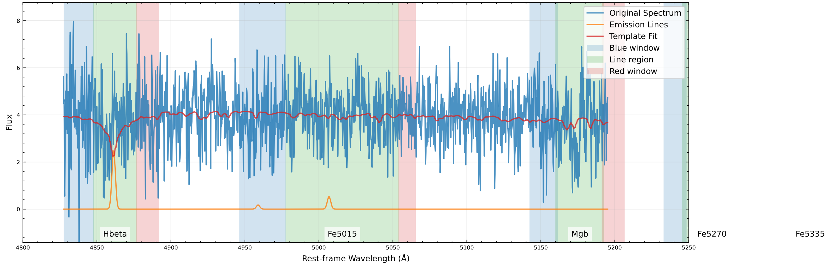
Original Data Comparison (v_star=25.8 km/s, v_gas=31.9 km/s)
