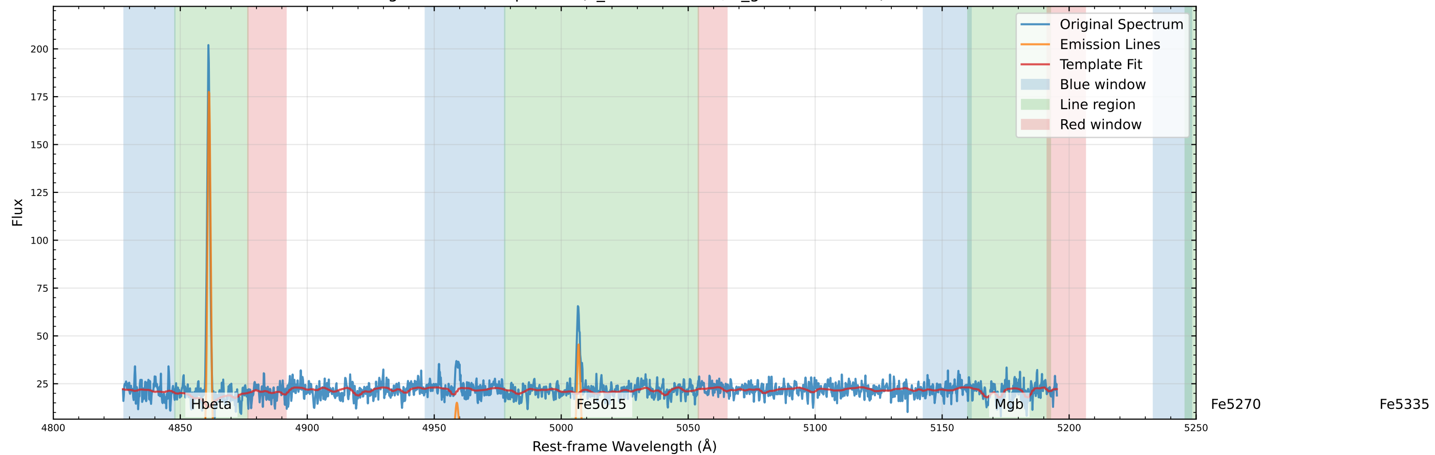
Original Data Comparison (v_star=2.0 km/s, v_gas=-10.9 km/s)
