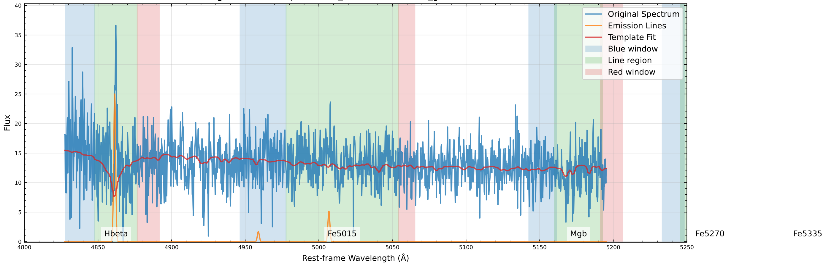
Original Data Comparison (v_star=25.0 km/s, v_gas=47.2 km/s)
