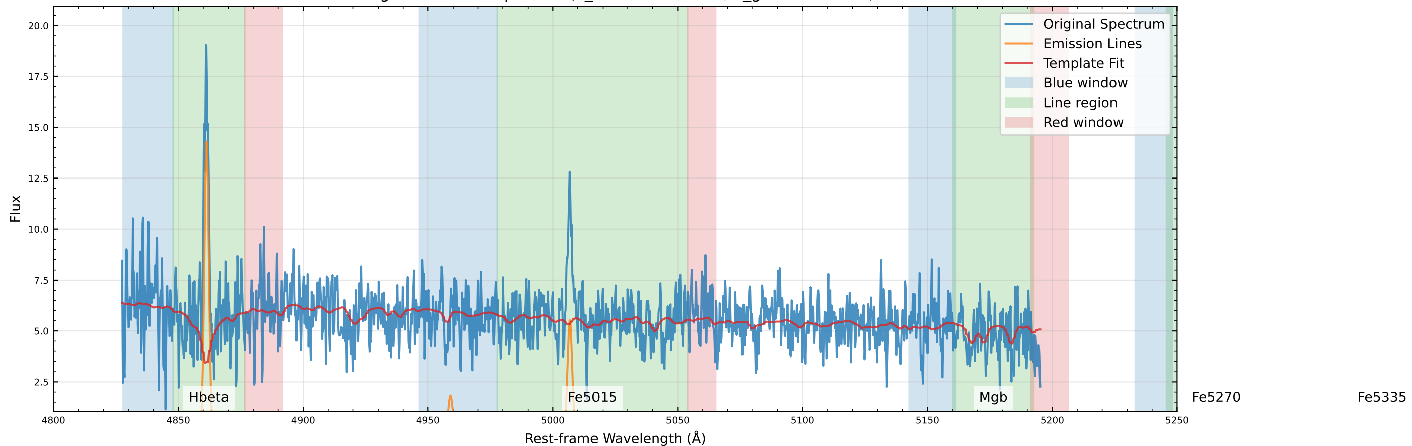
Original Data Comparison (v_star=-21.8 km/s, v_gas=-6.0 km/s)
