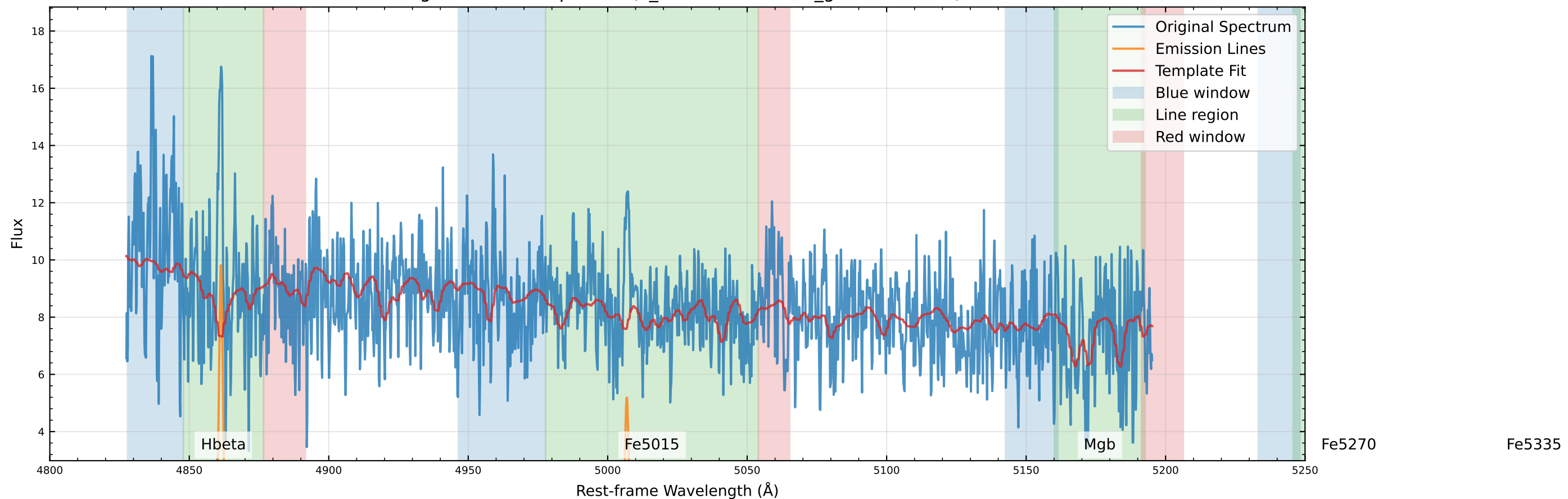
Original Data Comparison (v_star=-1.9 km/s, v_gas=-7.1 km/s)
