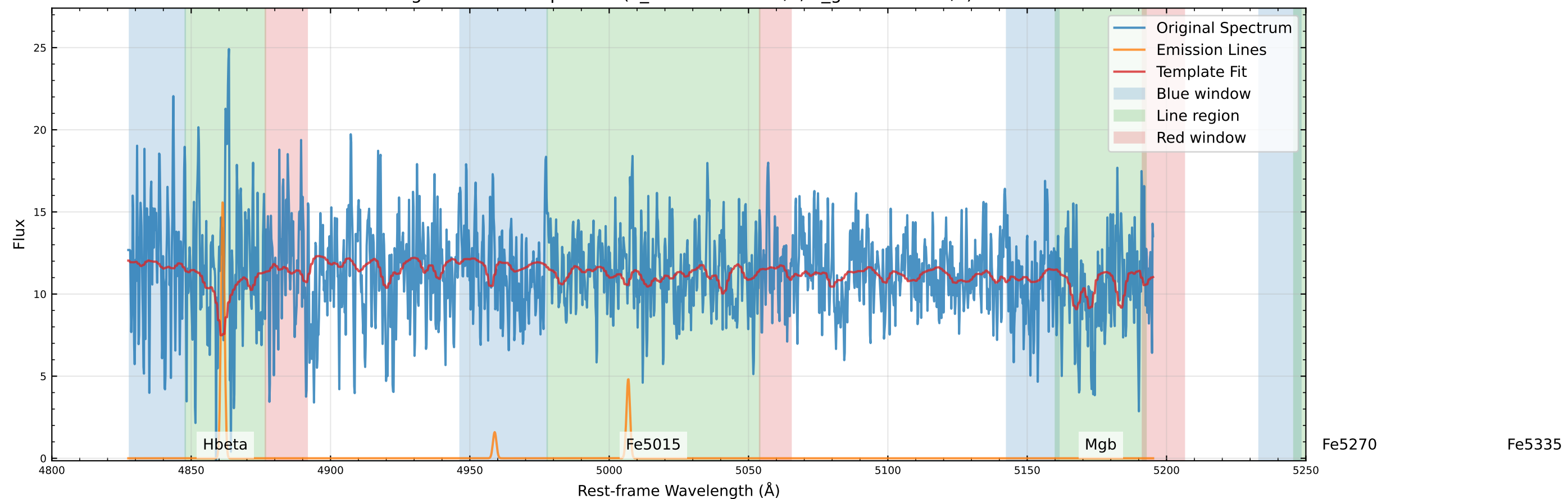
Original Data Comparison (v_star=100.1 km/s, v_gas=94.2 km/s)
