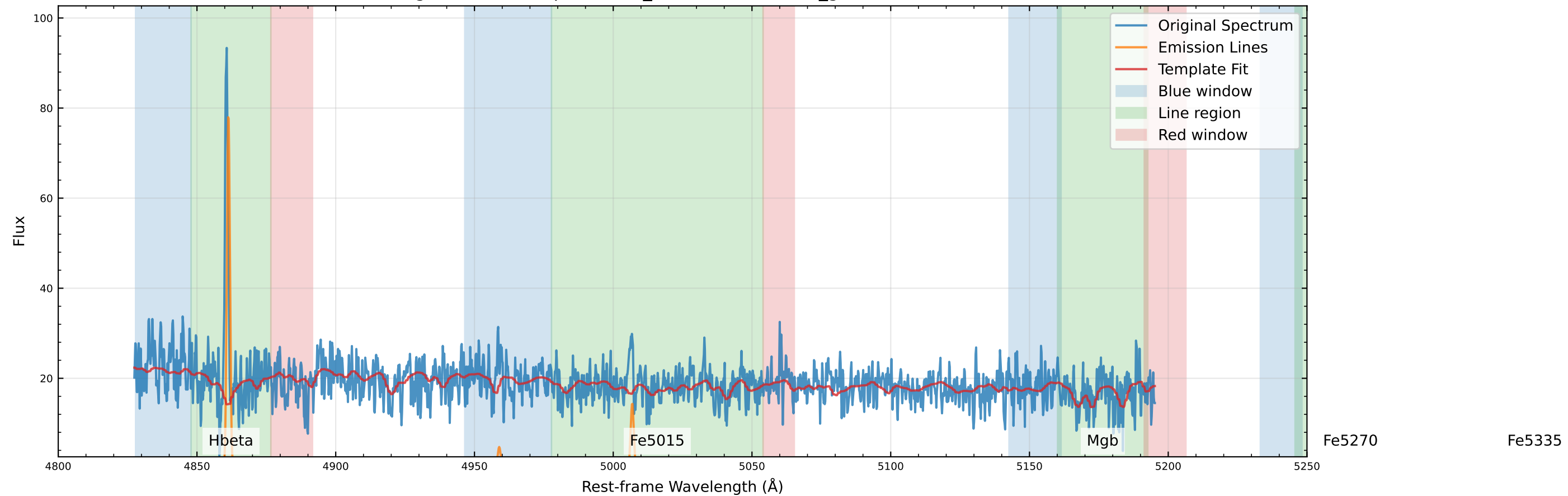
Original Data Comparison (v_star=-39.4 km/s, v_gas=-41.8 km/s)
