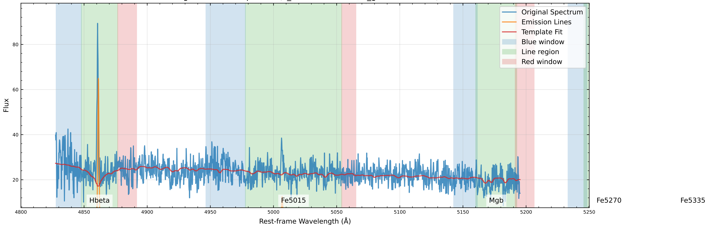
Original Data Comparison (v_star=-42.8 km/s, v_gas=-37.1 km/s)
