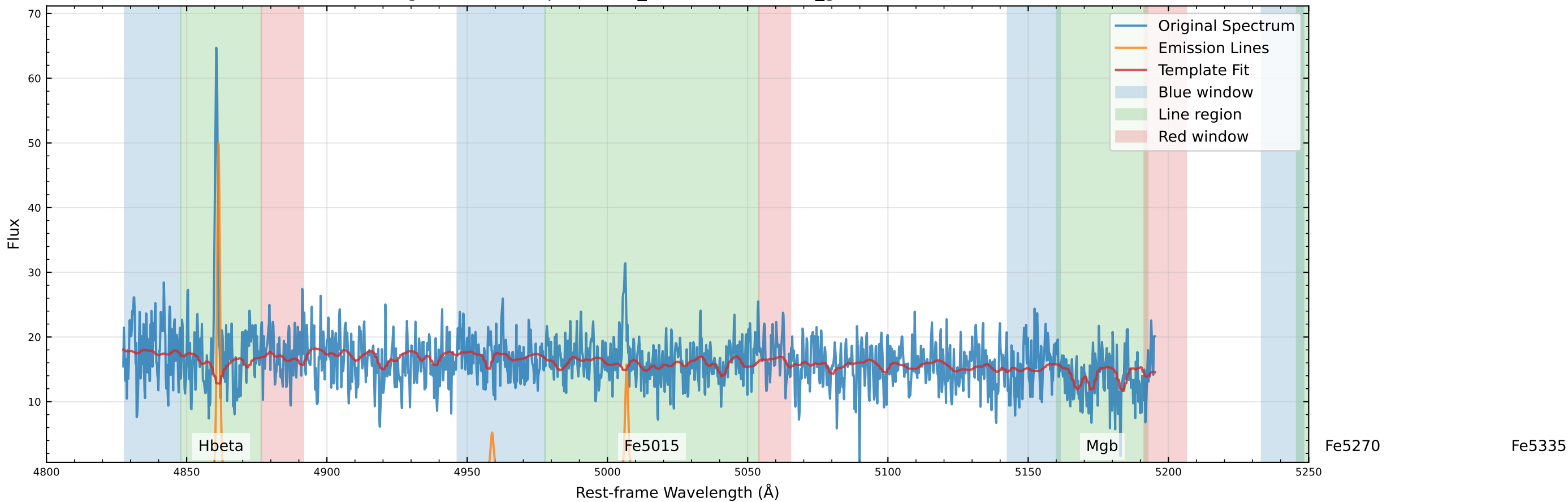
Original Data Comparison (v_star=-50.6 km/s, v_gas=-46.6 km/s)
