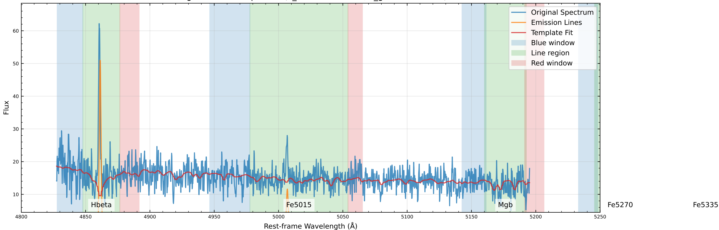
Original Data Comparison (v_star=-15.3 km/s, v_gas=-39.9 km/s)
