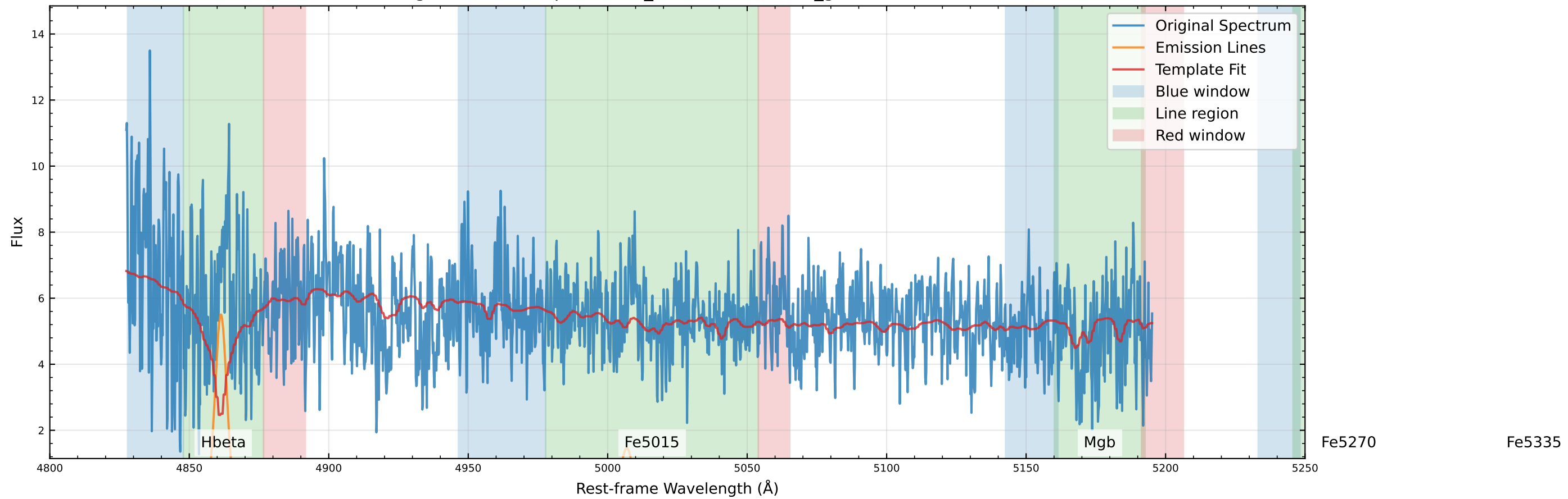
Original Data Comparison (v_star=25.2 km/s, v_gas=79.2 km/s)
