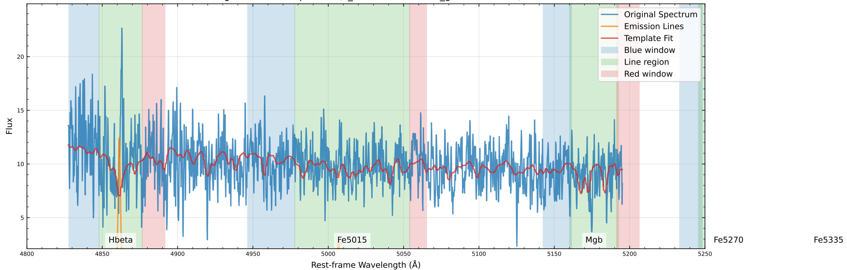
Original Data Comparison (v_star=76.4 km/s, v_gas=86.6 km/s)
