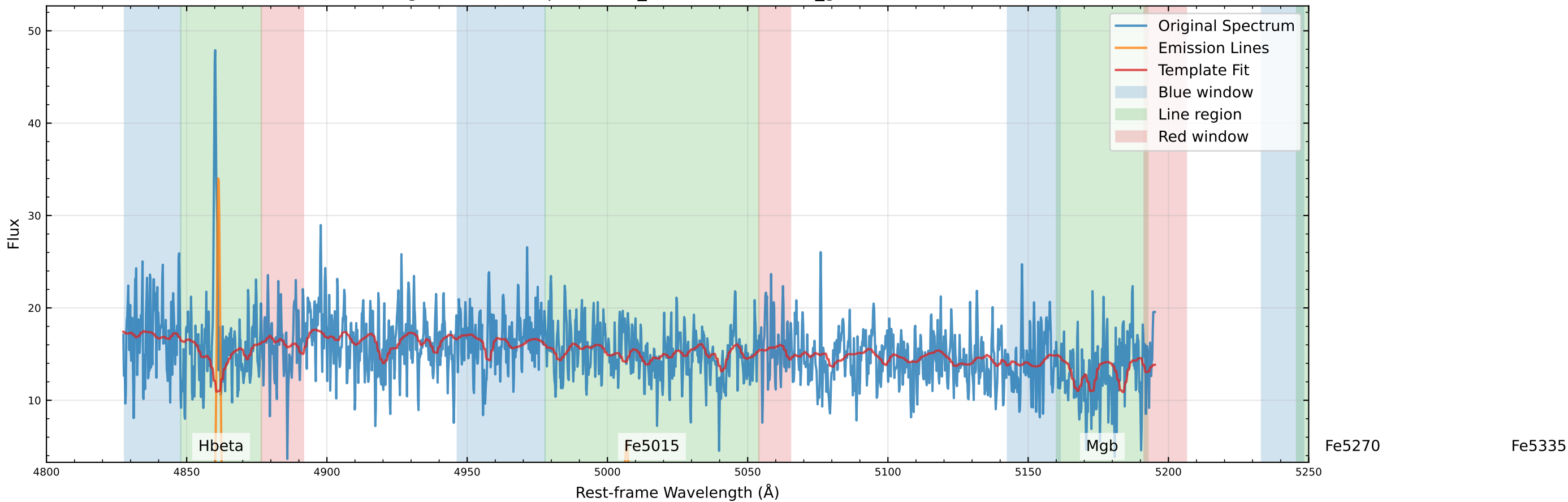
Original Data Comparison (v_star=-81.6 km/s, v_gas=-71.1 km/s)
