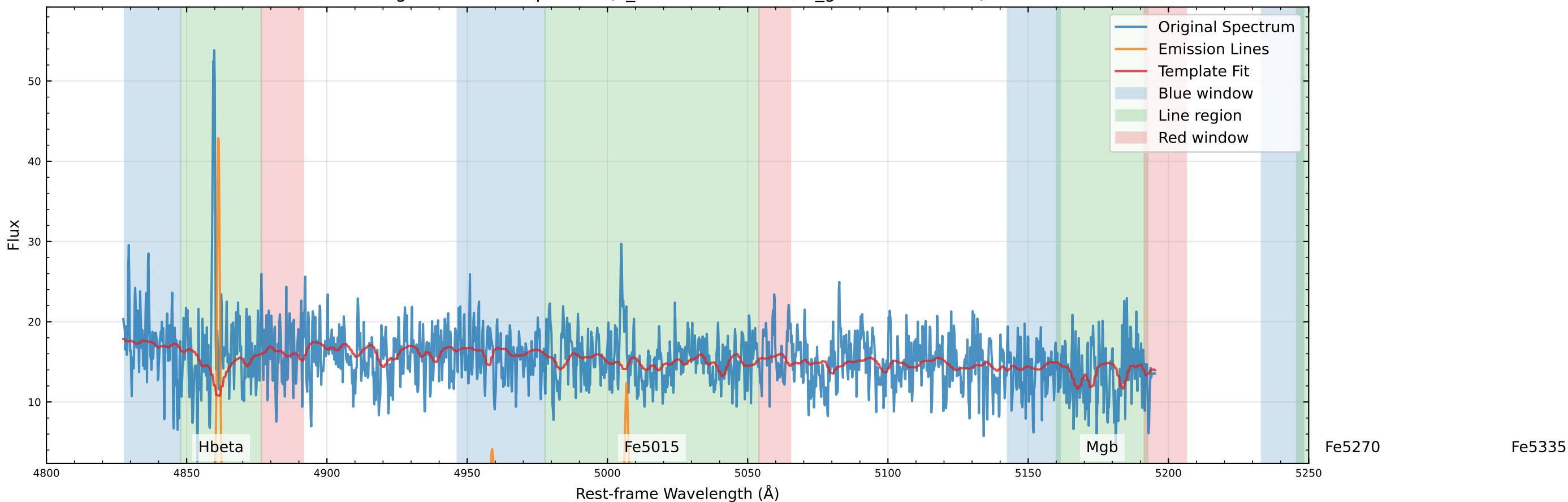
Original Data Comparison (v_star=-137.5 km/s, v_gas=-104.3 km/s)
