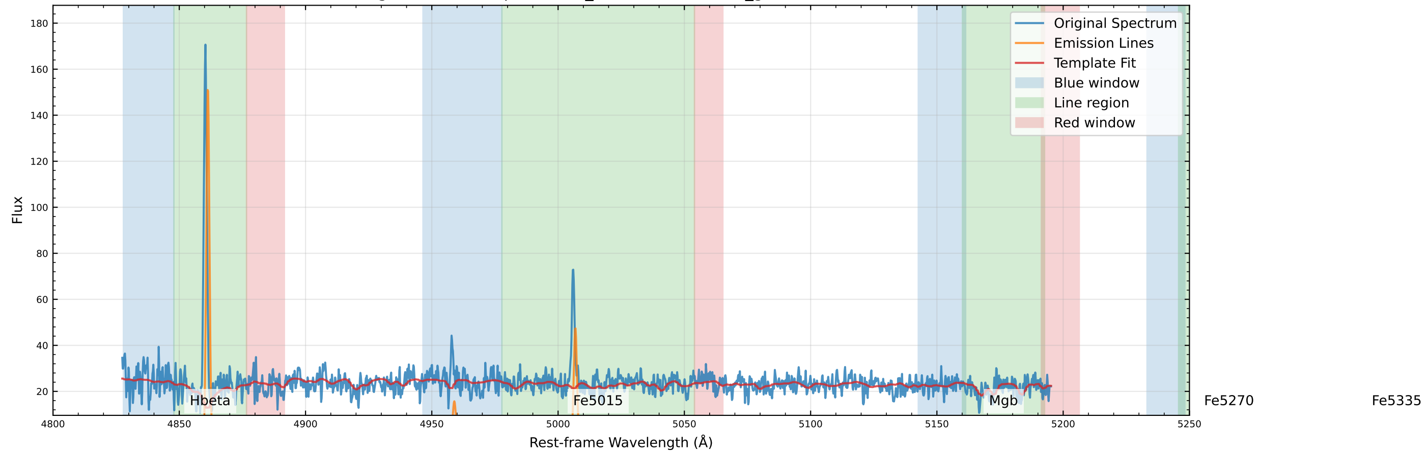
Original Data Comparison (v_star=-72.8 km/s, v_gas=-61.8 km/s)
