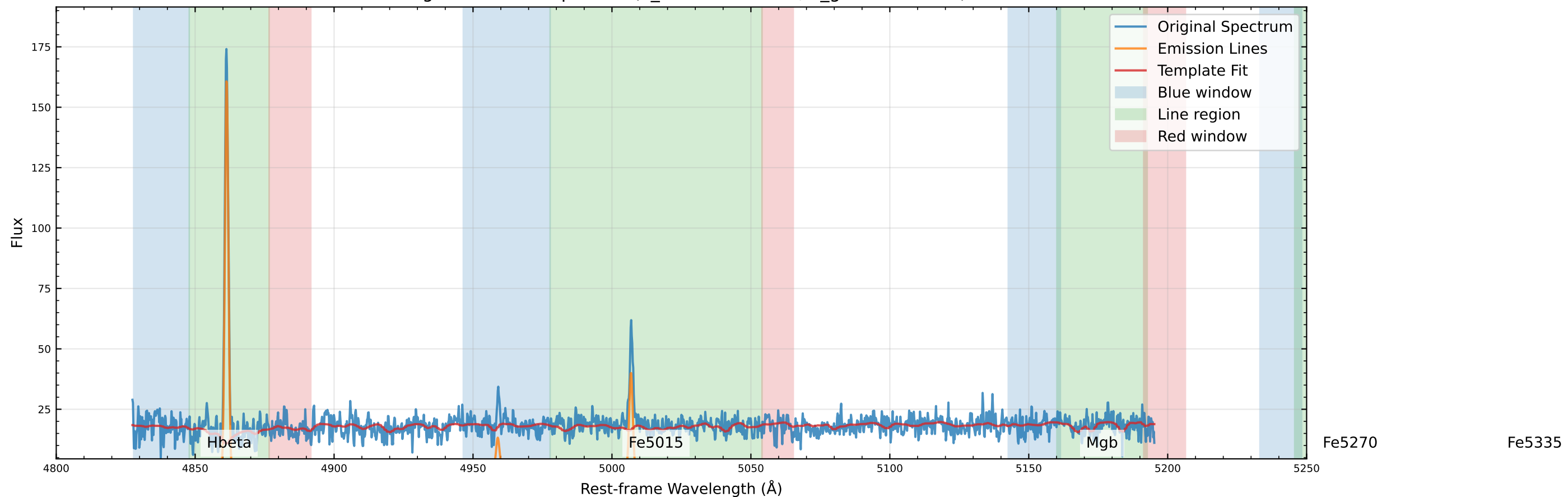
Original Data Comparison (v_star=17.6 km/s, v_gas=-2.7 km/s)
