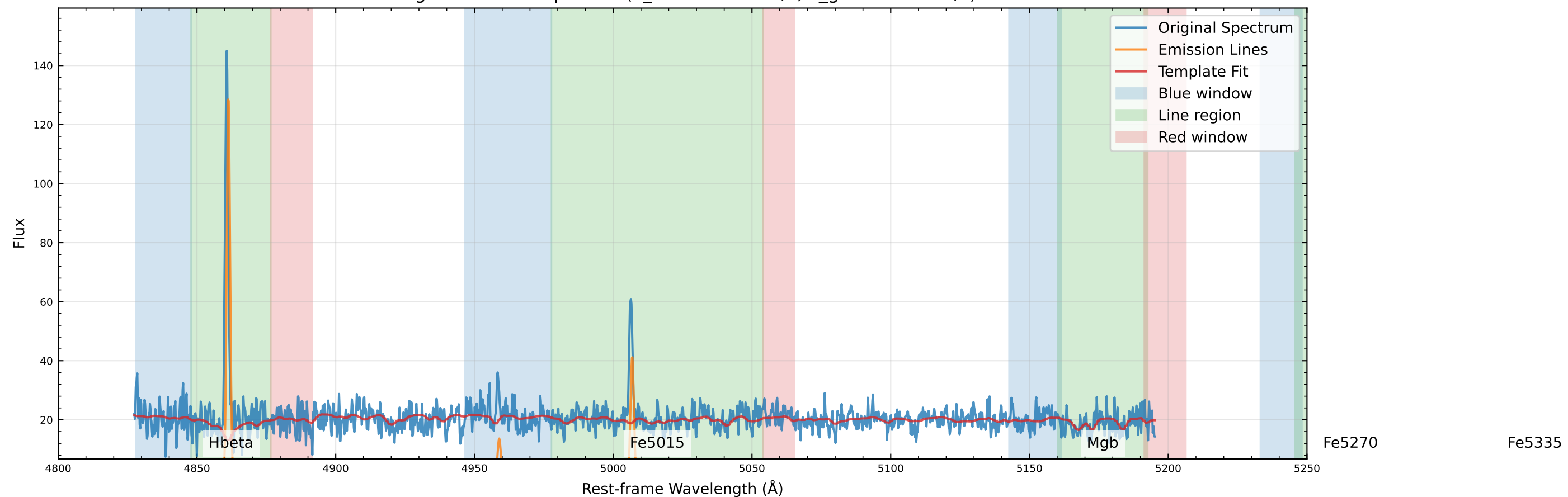
Original Data Comparison (v_star=-32.4 km/s, v_gas=-38.2 km/s)
