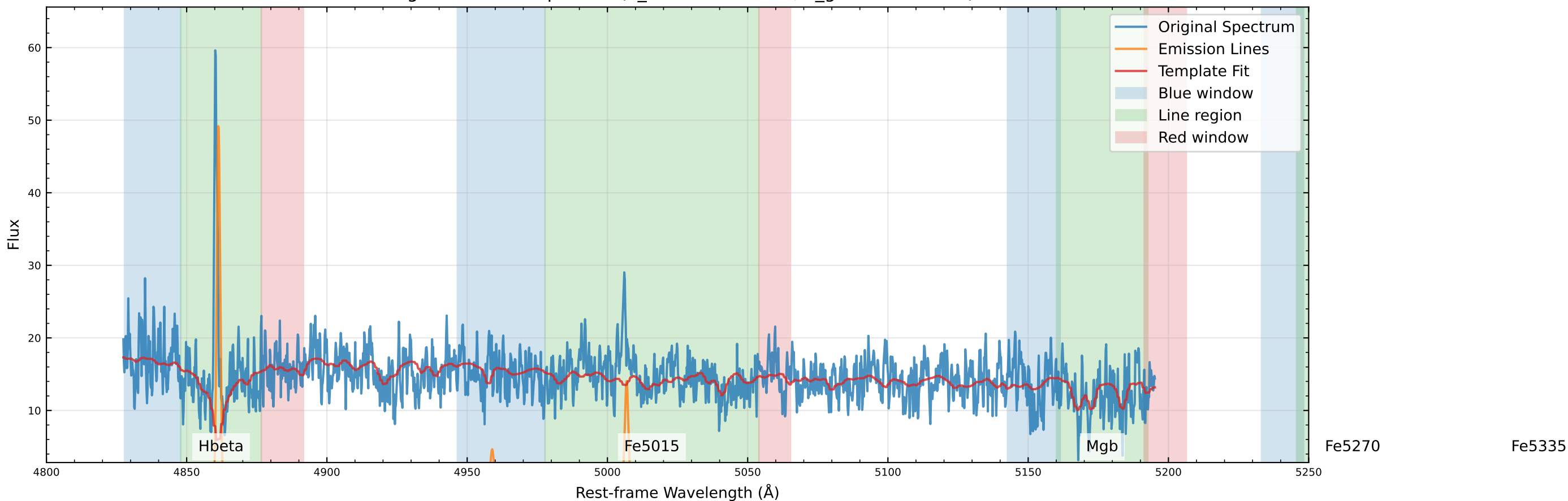
Original Data Comparison (v_star=-42.0 km/s, v_gas=-58.1 km/s)
