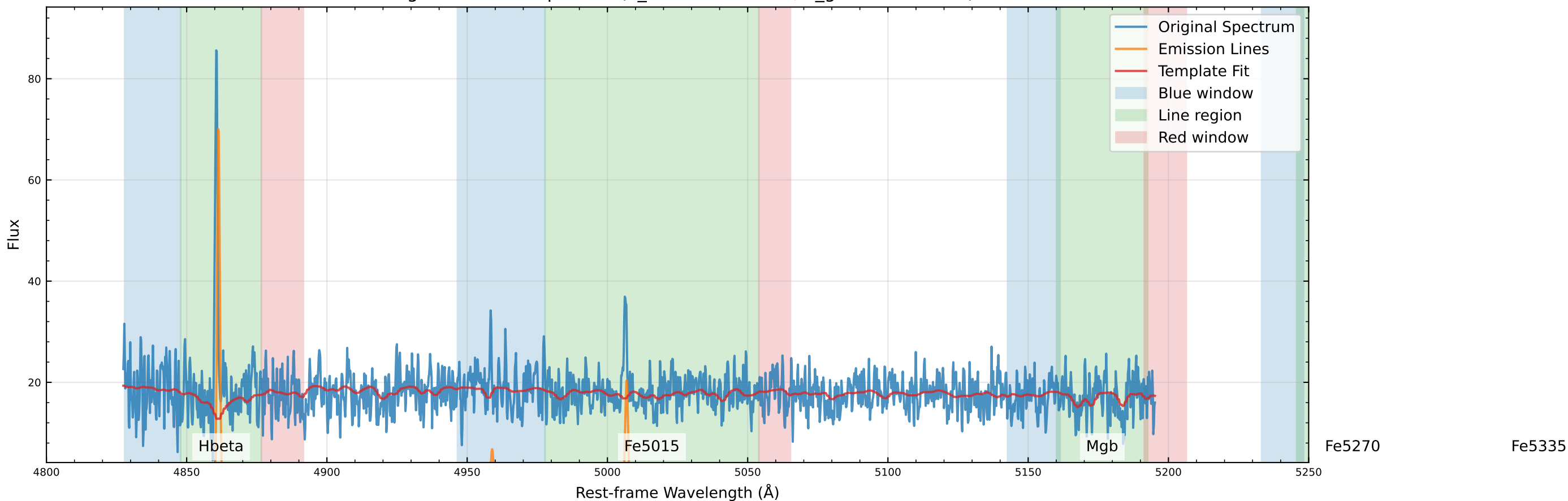
Original Data Comparison (v_star=-22.0 km/s, v_gas=-44.4 km/s)
