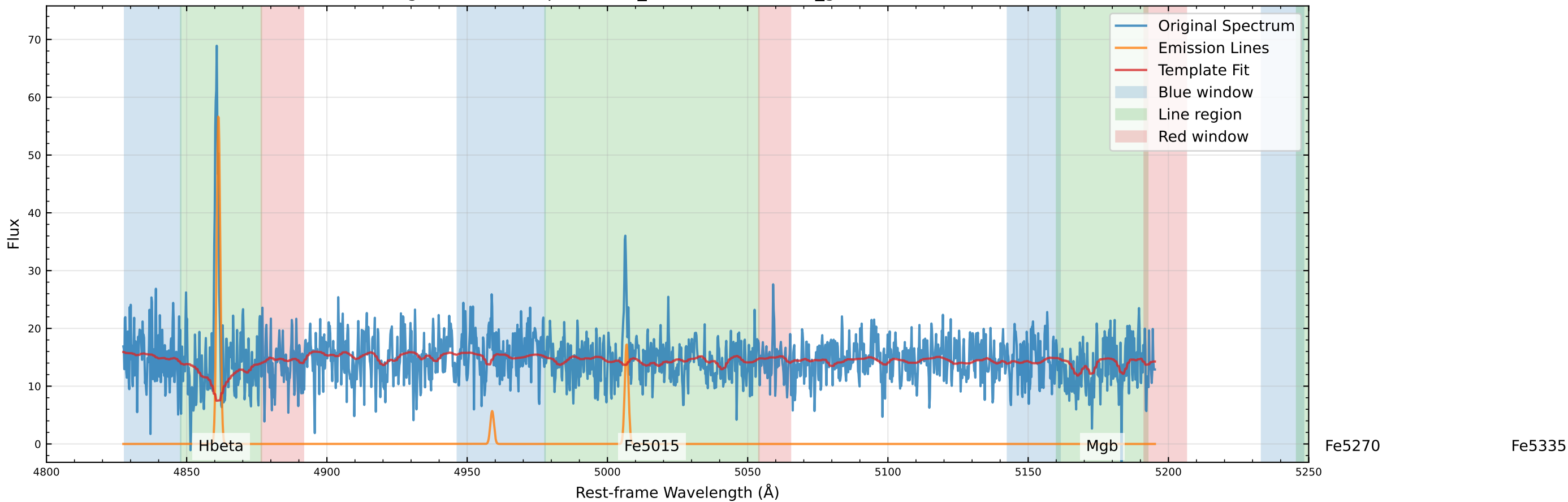
Original Data Comparison (v_star=-45.7 km/s, v_gas=-40.1 km/s)
