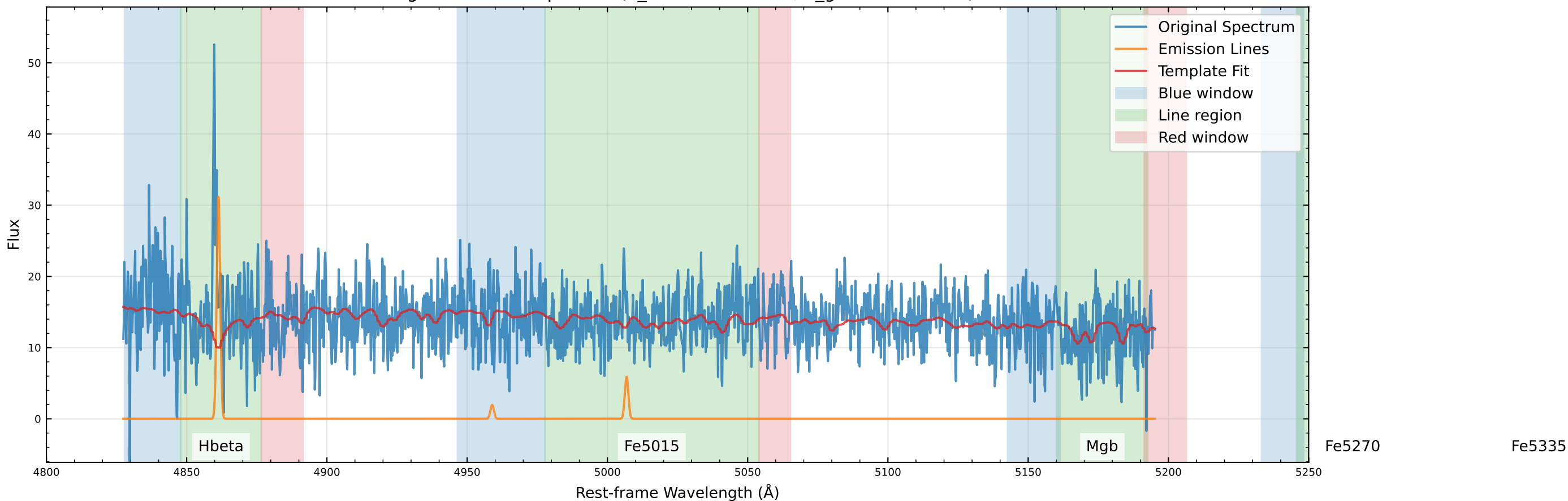
Original Data Comparison (v_star=-66.5 km/s, v_gas=-82.6 km/s)
