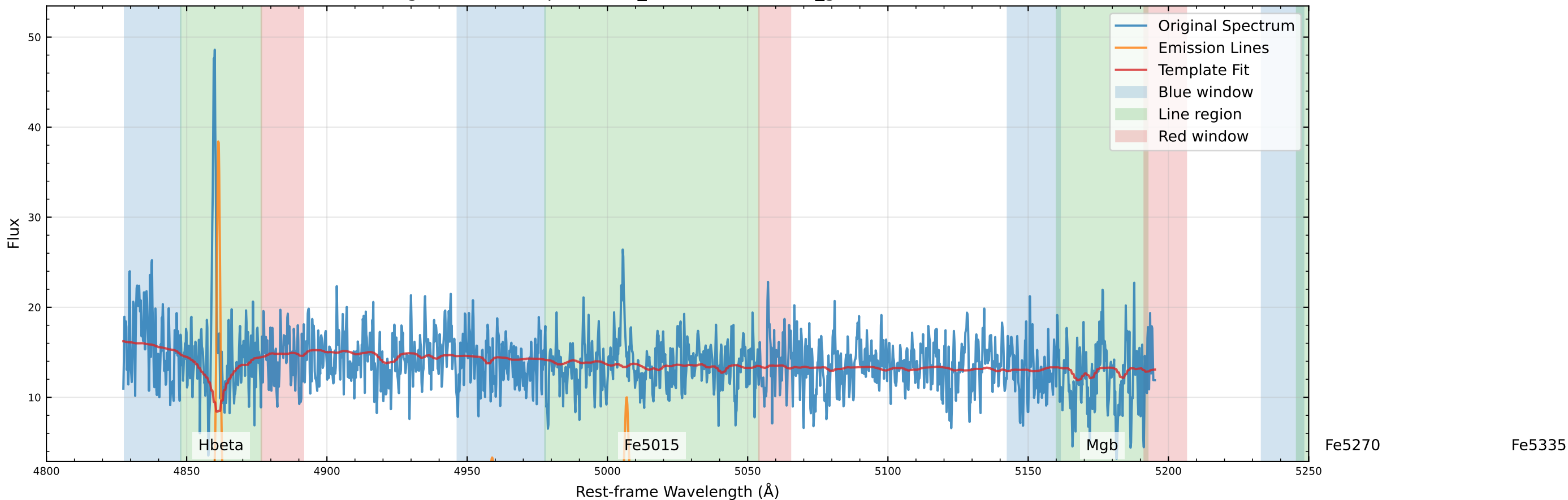
Original Data Comparison (v_star=-84.4 km/s, v_gas=-93.0 km/s)
