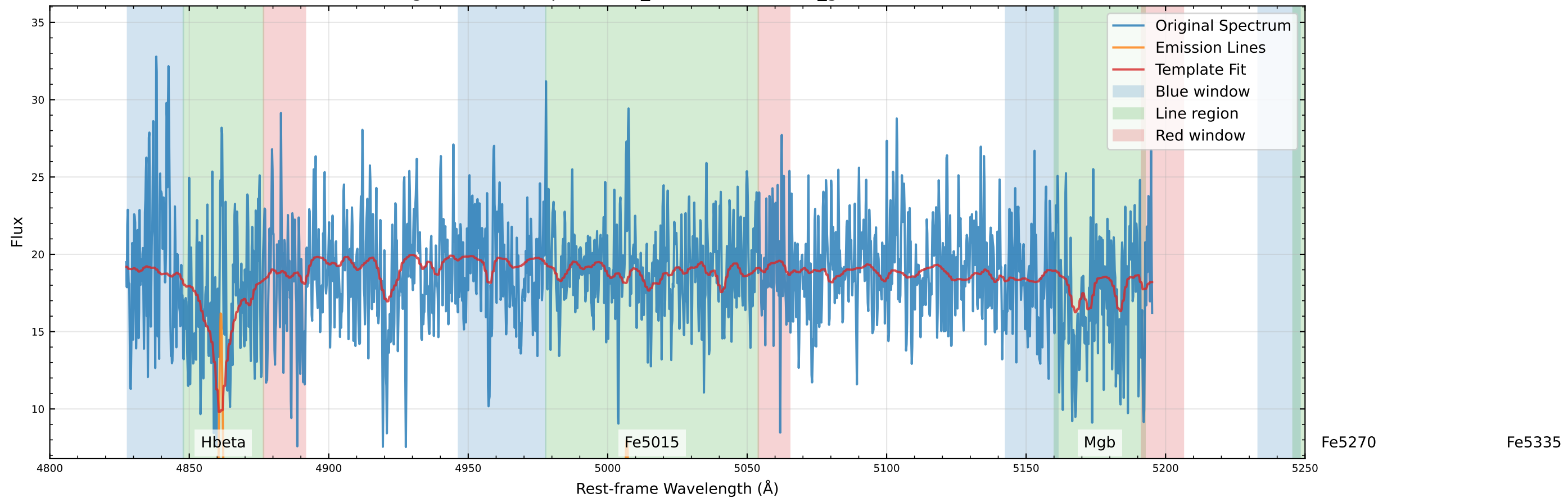
Original Data Comparison (v_star=-16.8 km/s, v_gas=12.7 km/s)
