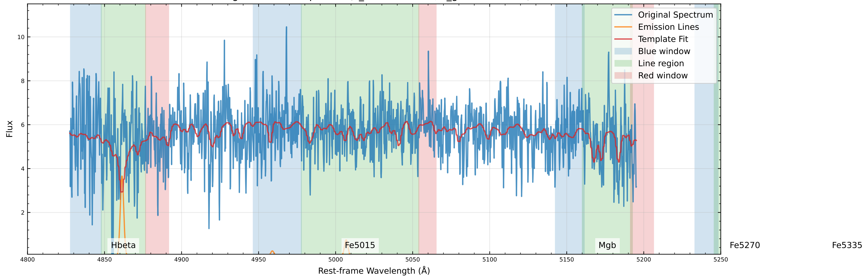
Original Data Comparison (v_star=8.6 km/s, v_gas=39.8 km/s)
