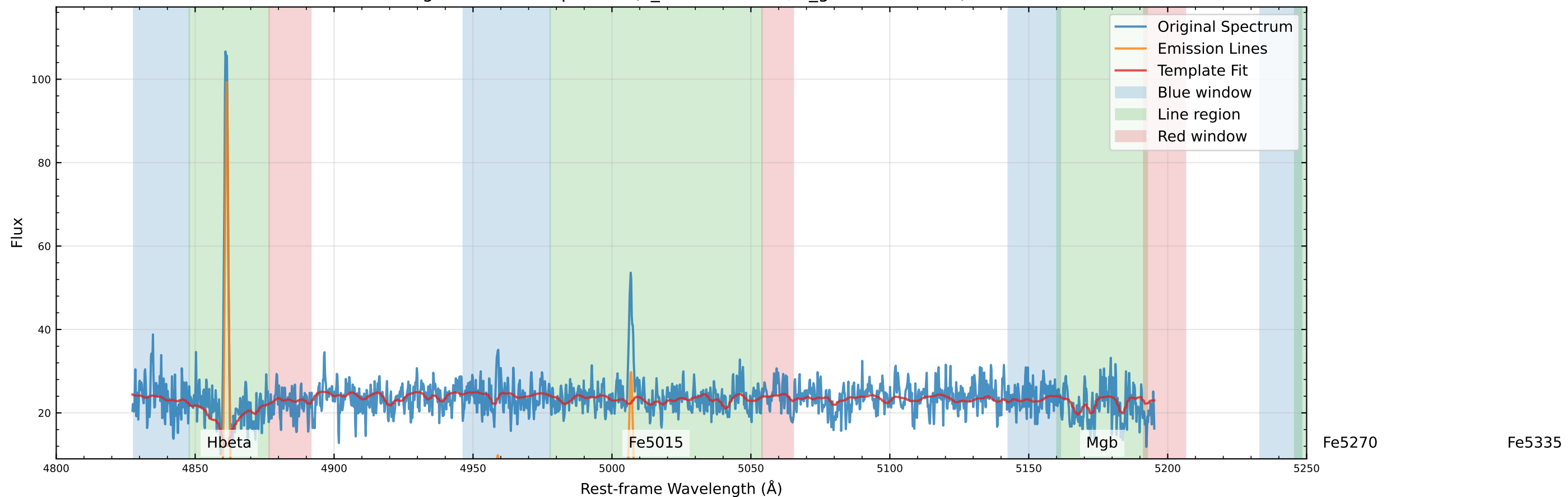
Original Data Comparison (v_star=2.1 km/s, v_gas=-10.4 km/s)
