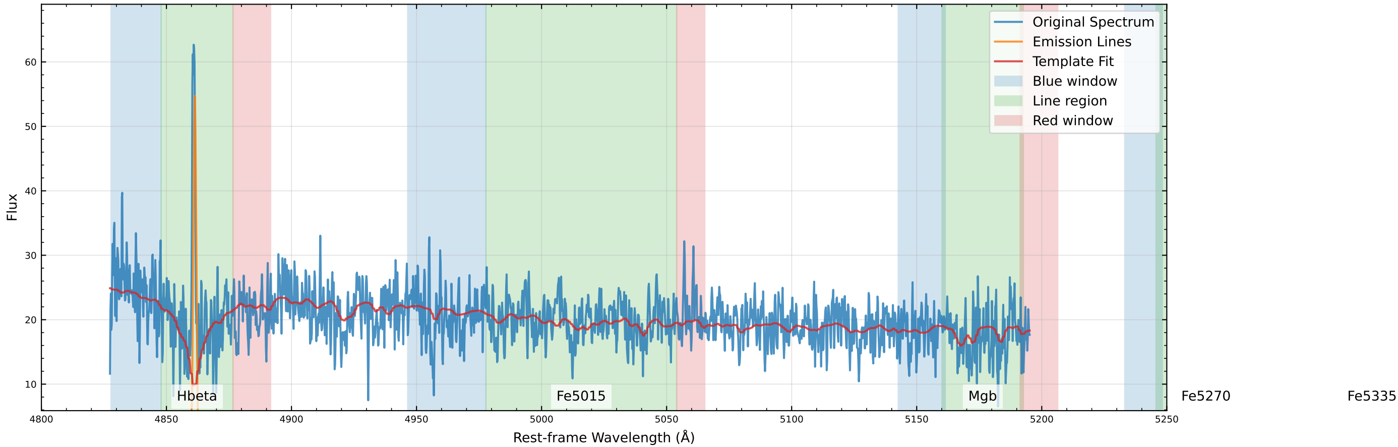
Original Data Comparison (v_star=-32.7 km/s, v_gas=-29.5 km/s)
