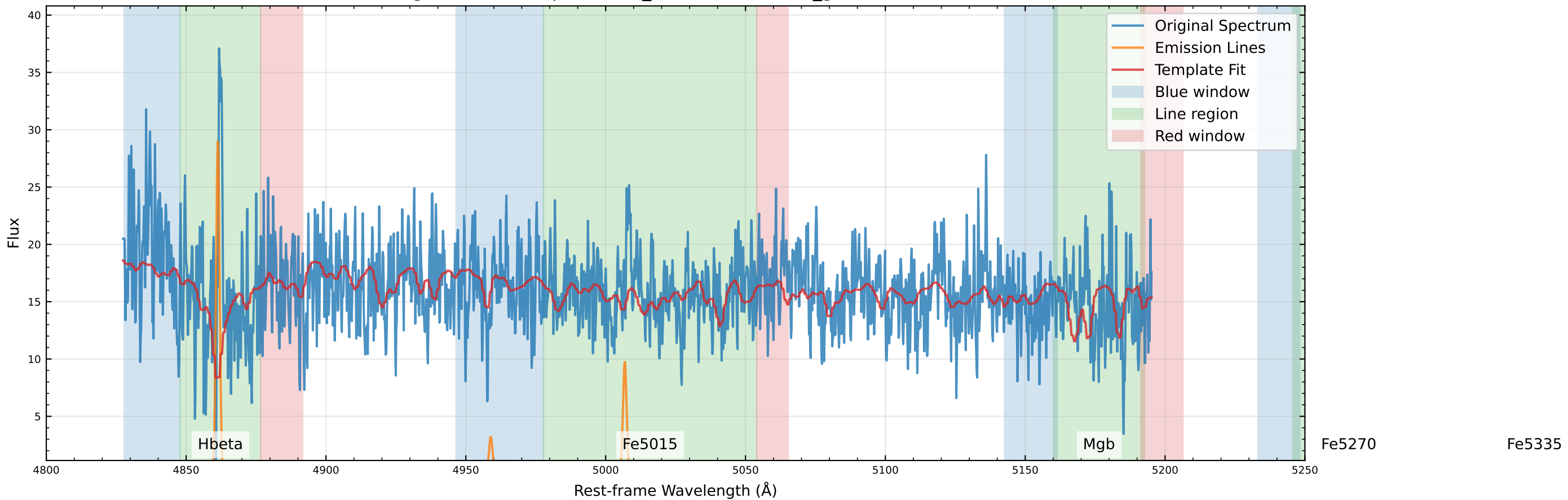
Original Data Comparison (v_star=77.1 km/s, v_gas=58.8 km/s)
