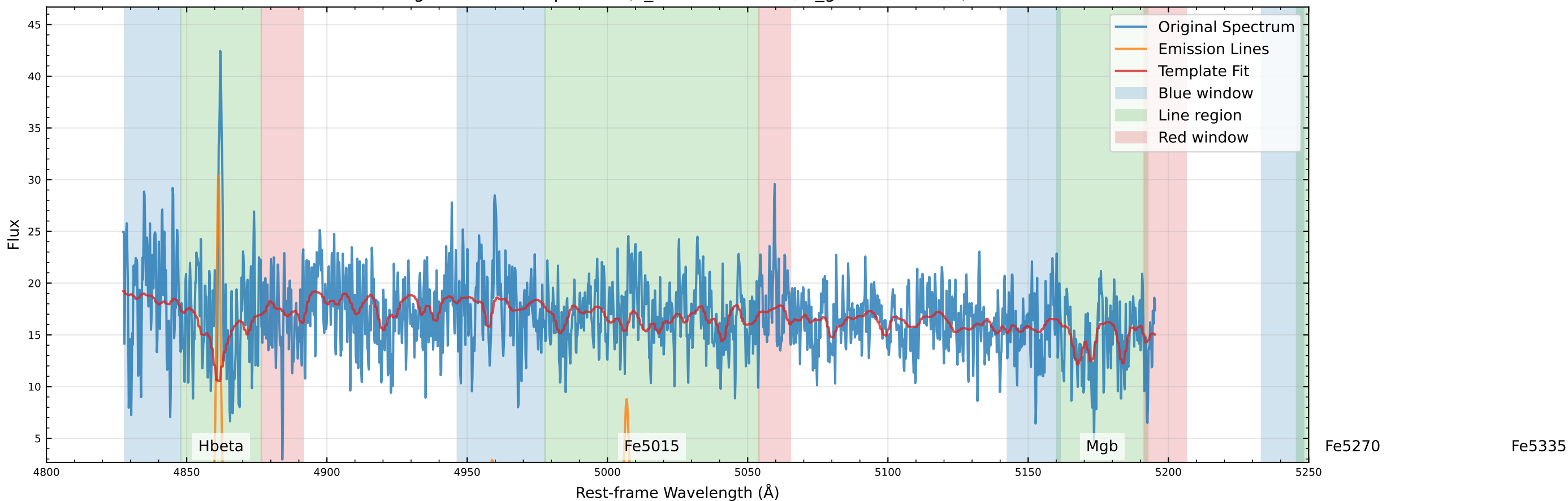
Original Data Comparison (v_star=27.9 km/s, v_gas=44.4 km/s)
