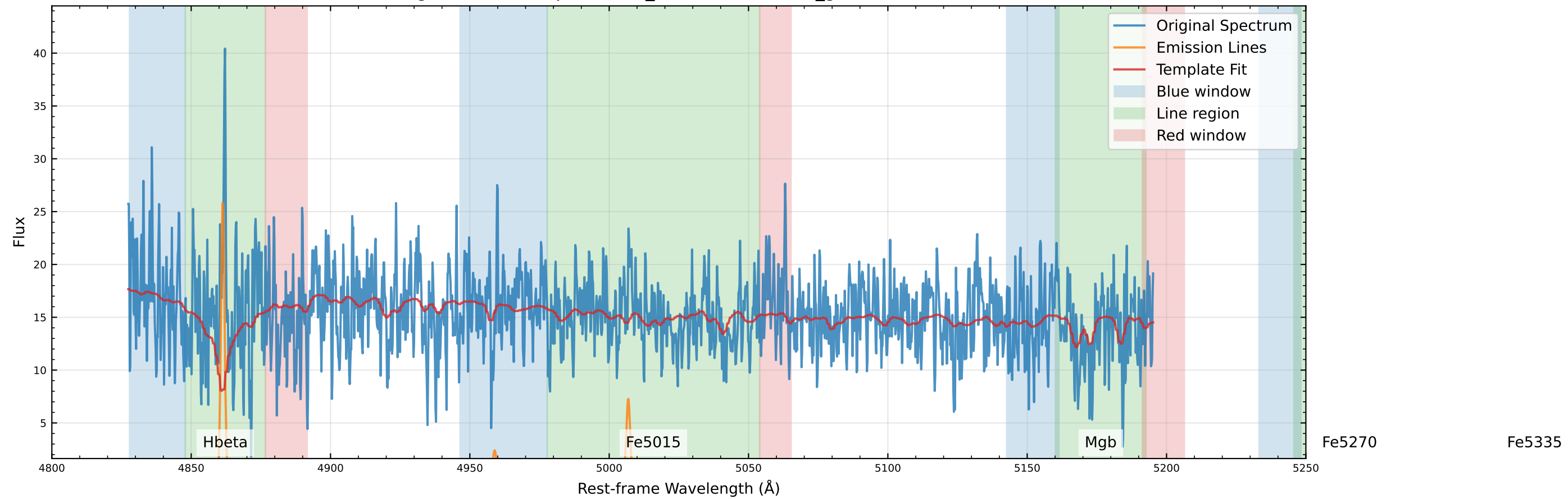
Original Data Comparison (v_star=32.8 km/s, v_gas=36.1 km/s)
