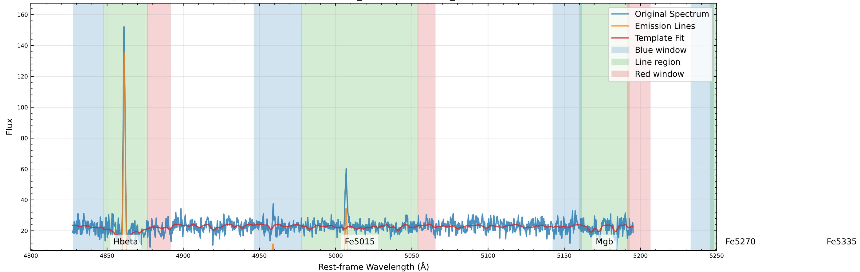
Original Data Comparison (v_star=13.4 km/s, v_gas=-6.6 km/s)
