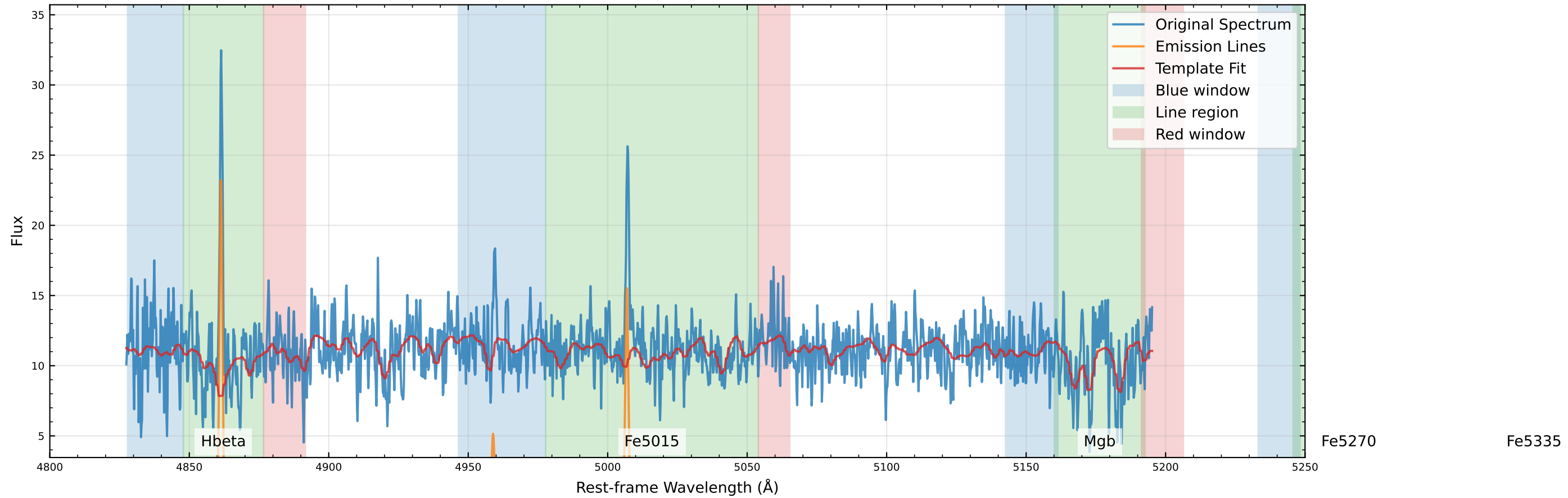
Original Data Comparison (v_star=-3.1 km/s, v_gas=10.5 km/s)
