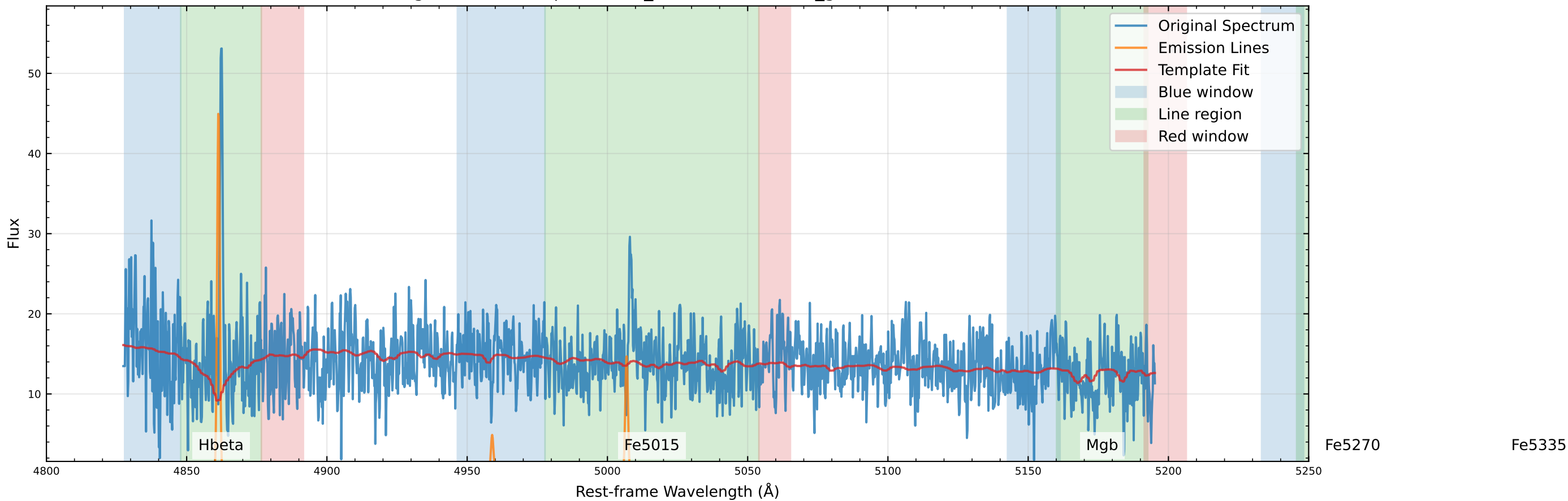
Original Data Comparison (v_star=67.0 km/s, v_gas=65.1 km/s)
