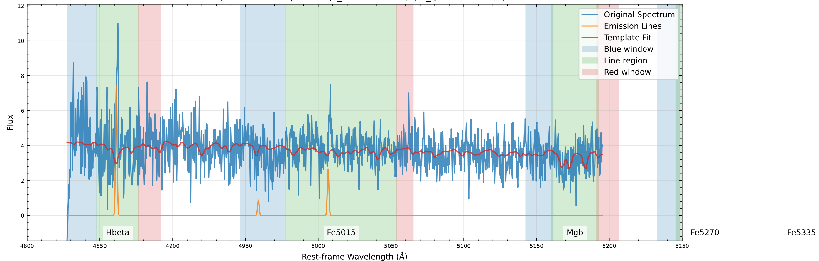
Original Data Comparison (v_star=56.6 km/s, v_gas=55.5 km/s)
