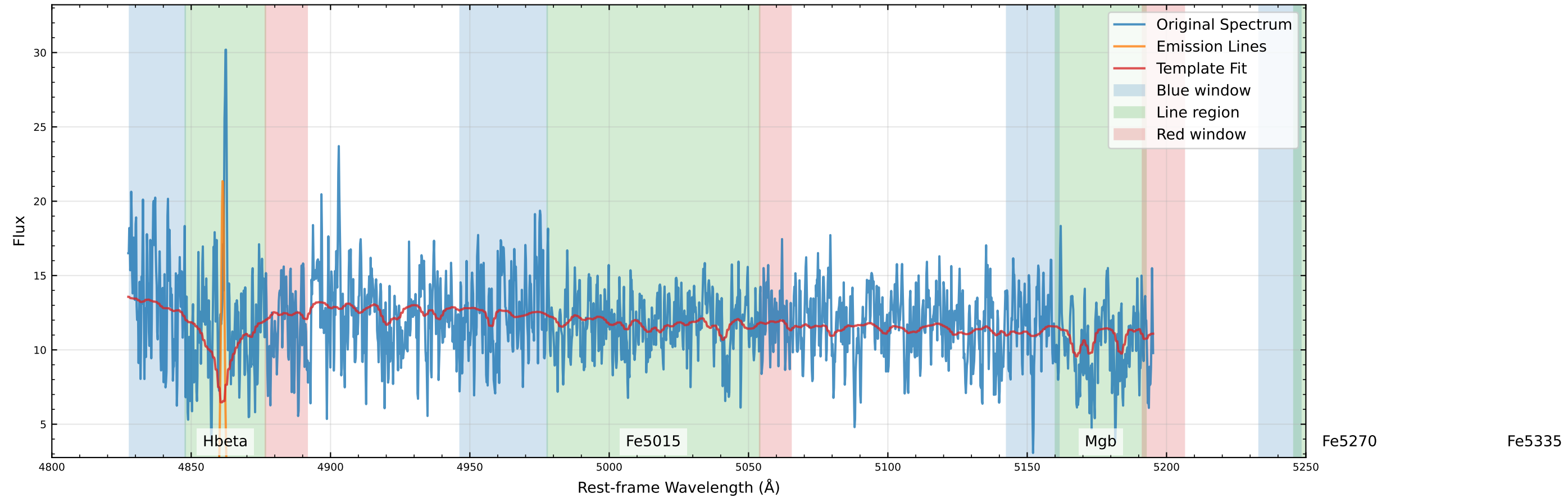
Original Data Comparison (v_star=46.6 km/s, v_gas=57.9 km/s)
