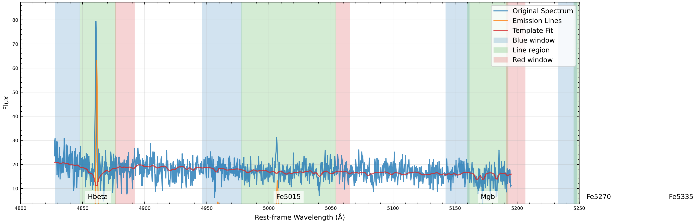
Original Data Comparison (v_star=-28.5 km/s, v_gas=-40.0 km/s)
