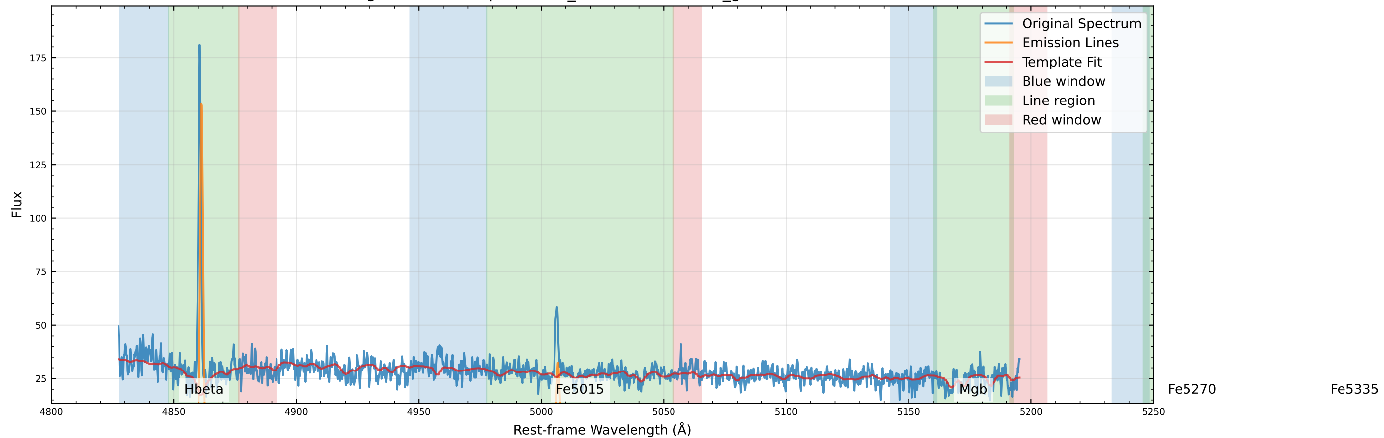
Original Data Comparison (v_star=-30.6 km/s, v_gas=-47.1 km/s)
