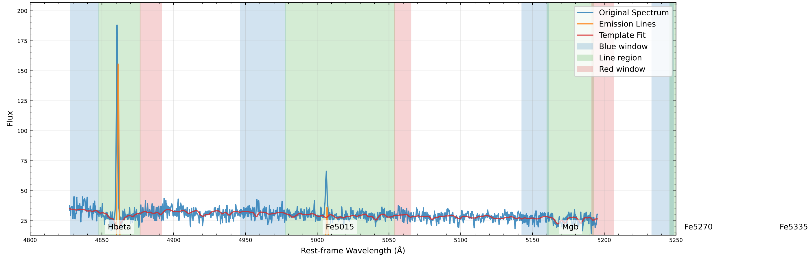
Original Data Comparison (v_star=-29.9 km/s, v_gas=-47.0 km/s)
