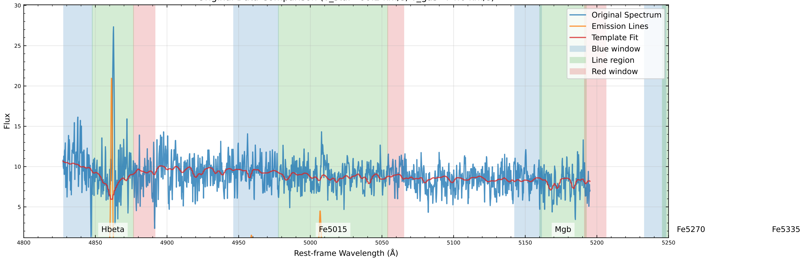
Original Data Comparison (v_star=60.2 km/s, v_gas=74.6 km/s)
