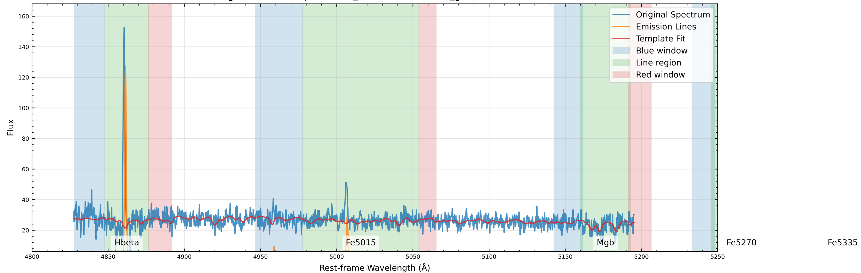
Original Data Comparison (v_star=-45.8 km/s, v_gas=-57.3 km/s)
