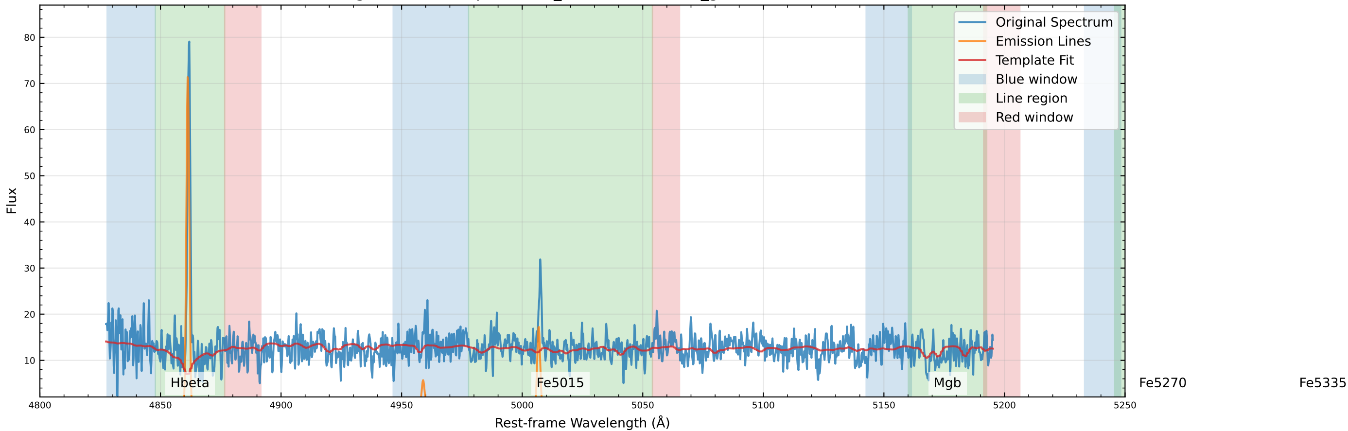
Original Data Comparison (v_star=49.5 km/s, v_gas=29.3 km/s)
