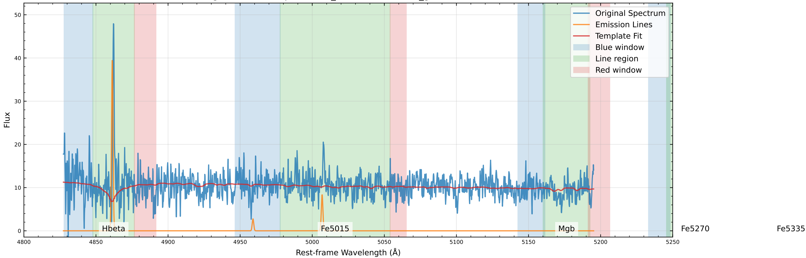
Original Data Comparison (v_star=61.2 km/s, v_gas=51.8 km/s)
