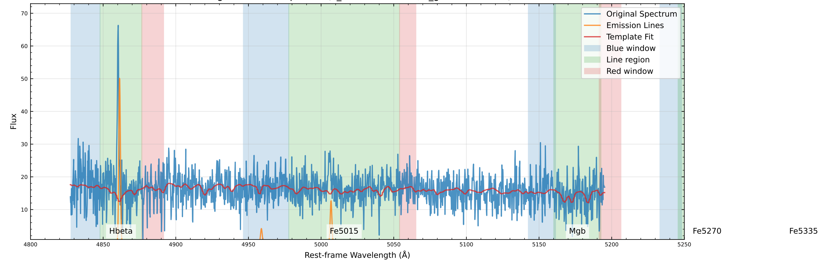
Original Data Comparison (v_star=-46.3 km/s, v_gas=-67.1 km/s)
