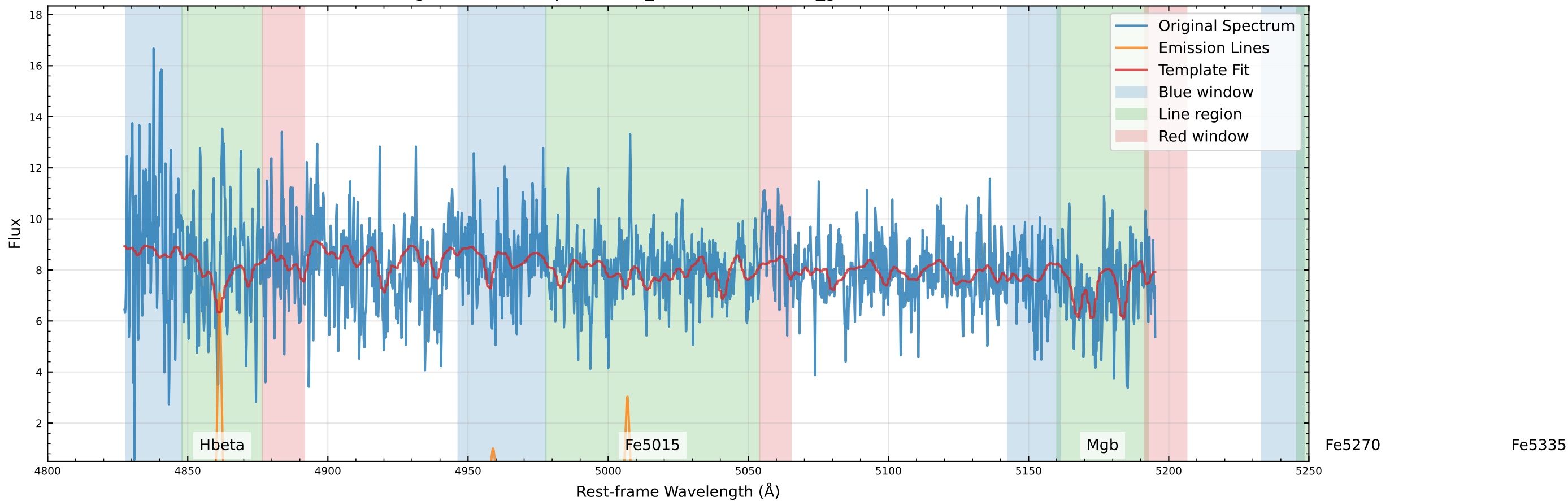
Original Data Comparison (v_star=49.4 km/s, v_gas=69.5 km/s)
