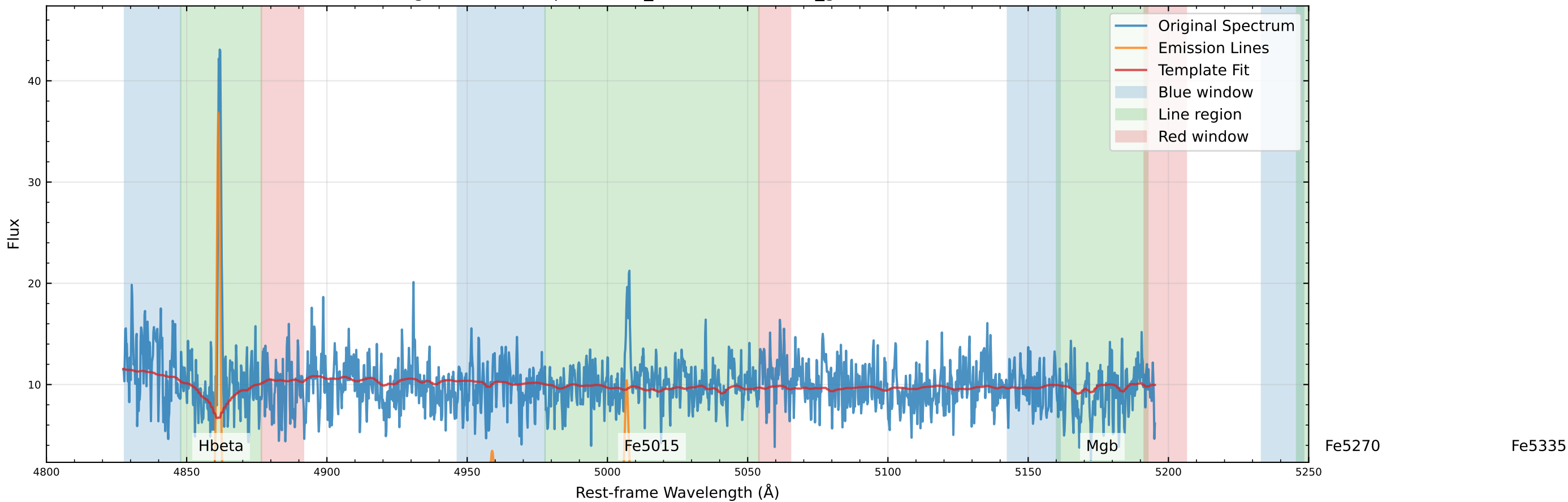
Original Data Comparison (v_star=31.8 km/s, v_gas=27.0 km/s)
