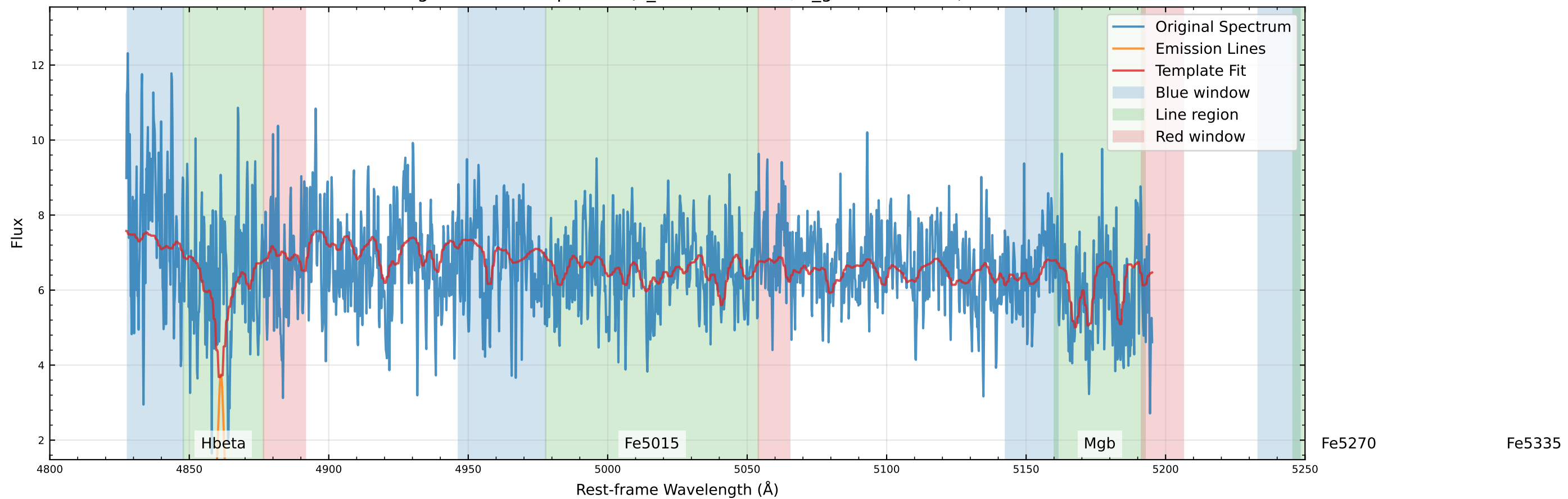
Original Data Comparison (v_star=-5.0 km/s, v_gas=13.9 km/s)
