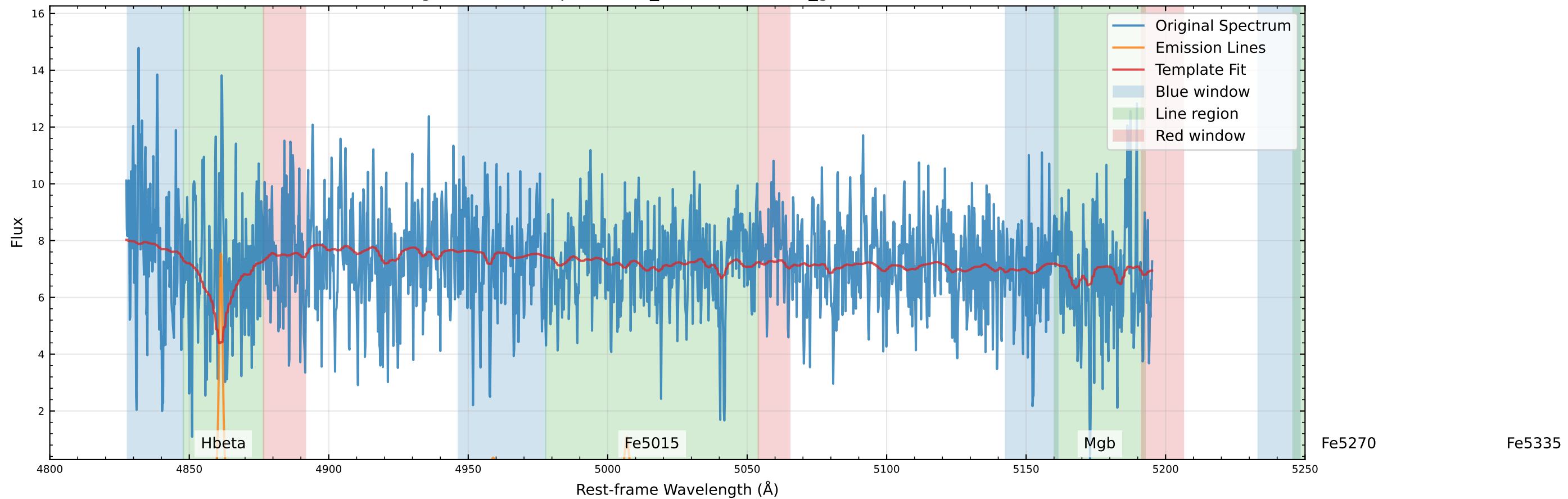
Original Data Comparison (v_star=4.6 km/s, v_gas=16.0 km/s)
